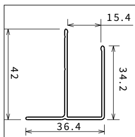
Standard profile 2P-G-B-S-S2-3P-2A
