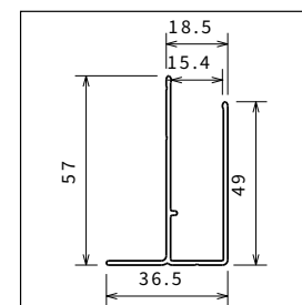
Extension Profile (Adds 15 mm)
