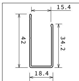
Standard profile A-R-F
